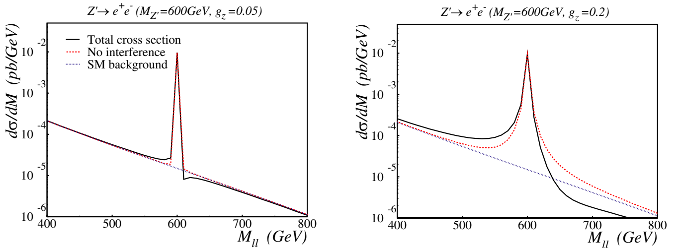
FIG. 9 (color online). NLO differential cross sections for the production of electron-positron pairs as a function of the invariant mass of the pair, in the U(1)_{B+L} model. The solid curves correspond to the total cross sections for the signal, including interference terms, for the gauge coupling fixed to g_z = 0.05 and g_z = 0.2 respectively. Dashed lines are the same cross sections neglecting interference terms and the dotted lines correspond to the SM background.
