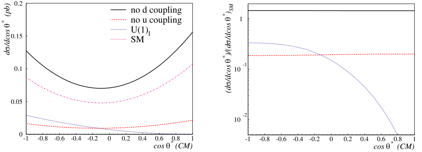
FIG. 5 (color online). (a) Angular distribution, in the CM frame of the lepton pair, at LO in QCD for different models. The lines labeled no u ( d ) coupling correspond to SM charges but neglecting the coupling of up (down) type quarks to the Z' . (b) Ratio between the differential cross section (shown in panel a) in different models and the case of SM-like charges.
