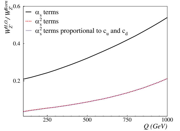
FIG. 3 (color online). The ratio of the \mathcal{O}(\alpha_s) and \mathcal{O}(\alpha_s^2) corrections to the hadronic structure function over the Born contribution, assuming SM couplings for the Z' . The full line corresponds to the \mathcal{O}(\alpha_s) corrections. The dashed and dotted lines, which, within the resolution of the figure, appear as a single line, correspond to the total \mathcal{O}(\alpha_s^2) contributions and to the \mathcal{O}(\alpha_s^2) corrections retaining only those terms that give contributions proportional to c_u and c_d to the cross section, respectively.
