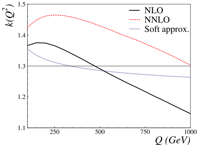
FIG. 4 (color online). NLO and NNLO k -factors for SM-like couplings as a function of the invariant mass of the lepton pair. Also shown is an approximation, Eq. (3.11), for the NLO k -factor which only takes into account the soft corrections to the structure function in the deeply inelastic scattering scheme.
