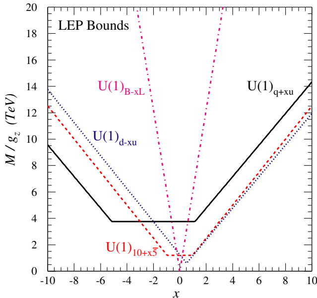
FIG. 1 (color online). Lower bounds on M_{Z'}/g_z from the LEP-II search for LL , RR , LR and RL contact interactions, applied to the models of Table I as a function of the continuous parameter x . For U(1)_{B-xL} , we have included the bound on vectorlike e^+e^- \rightarrow \ell^+\ell^- , as is appropriate for that model.
