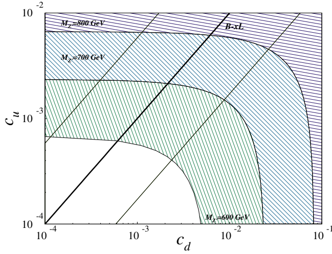
FIG. 2 (color online). Excluded regions in the c_d - c_u plane from the current 95% C.L. limit for \sigma \cdot \text{Br}(Z' \rightarrow l^+ l^-) given in [27], for different values of the Z' mass. The thick straight line corresponds to values of c_u and c_d in the B - xL model, in which c_u = c_d . The area between the two thin straight lines is the region where the q + xu model lies.
