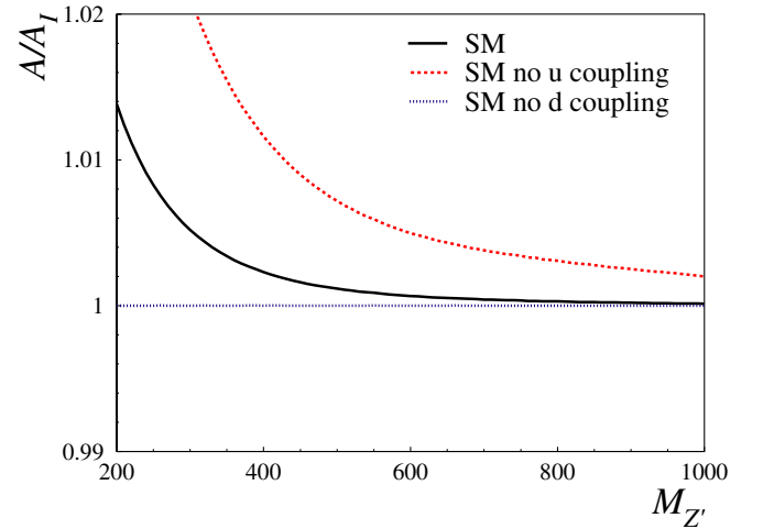
FIG. 6 (color online). The Acceptance ( A ), computed from the LO cross section integrated over the azimuthal angle of the leptons in the laboratory frame in the region 50^\circ \leq \theta_{\text{lab}} \leq 130^\circ . We considered the cases of SM couplings, SM couplings without u -quark couplings and without d -quark couplings, respectively. To show the variation compared to a most extreme situation, we normalize to the corresponding LO acceptance of the U(1)_I model.
